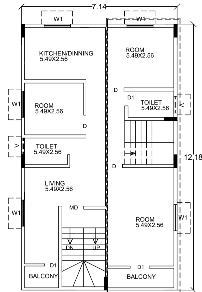
EX.FIRST FLOOR WITH PLAN ALTERATION
